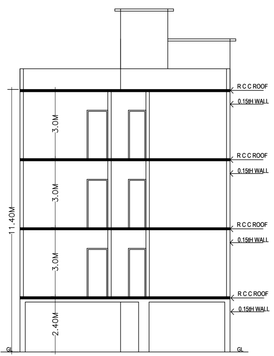
SECTION @ X-X
